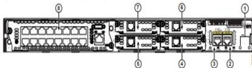
Figure 3 Cisco 2811 Rear Panel Physical Interfaces
