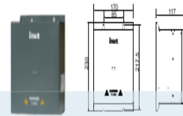
Installation dimension
