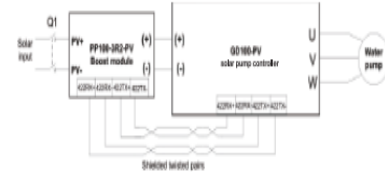
Connection between the boost module and solar pumping controller
